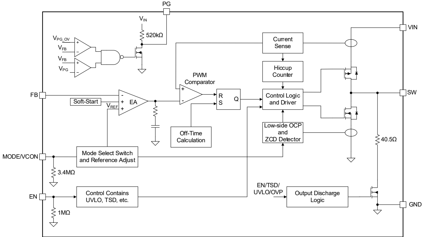
Figure 2. SGM61061 Block Diagram
