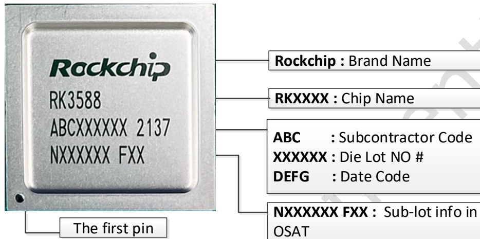
Fig.2-1 Package definition
